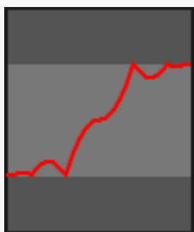
static in-out-circ(progress)
