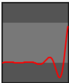
static in-expo(progress)
