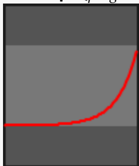
static in-out-back(progress)
