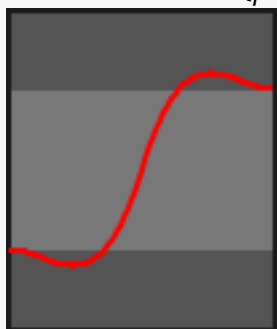
static in-out-bounce(progress)
